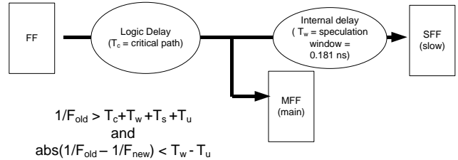
Figure 3. Timing requirements
