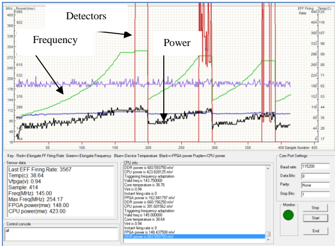
Figure 4. Monitoring tool screen capture.
