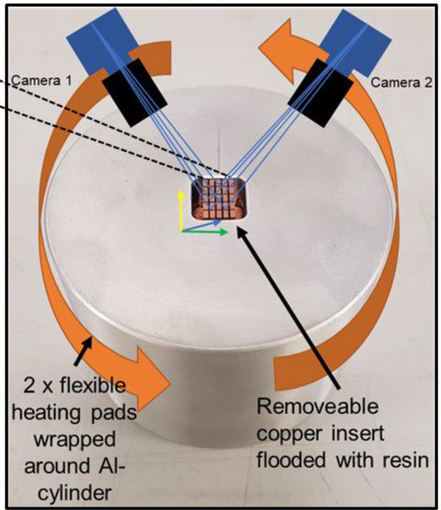
*Picture of experimental set-up
