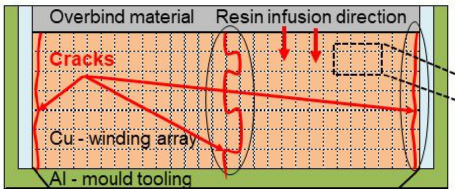
*Schematic of magnet manufacturing
